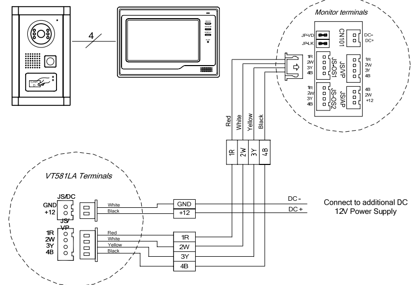
Wiring Diagram 2 (VT581L is powered by Additional +12V Adaptor)
